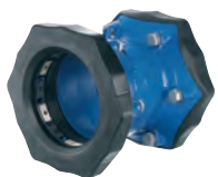
Series 631 Supa Maxi™ straight coupling Universal and tensile for all pipes DN50-800 PN16 Ductile iron
